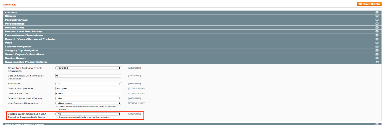
Figure 2: Catalog Settings
