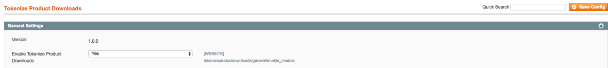
Figure 1: Configuration Settings
